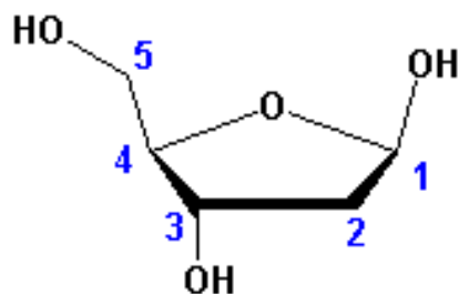
2-deoxyribose
