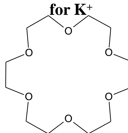
18-crown-6
